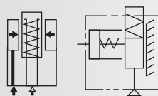
Work Support, Air Advance
