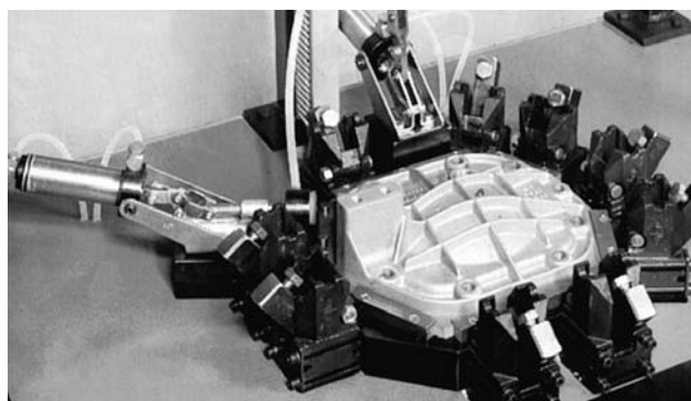
Power clamp models 871-2 and 803 on a pressure test fixture for vehicle gearbox lids
