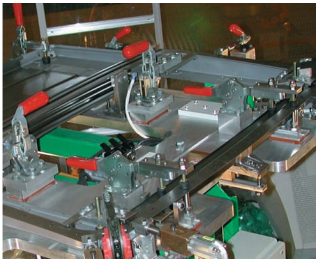
Manual Clamping Technology
