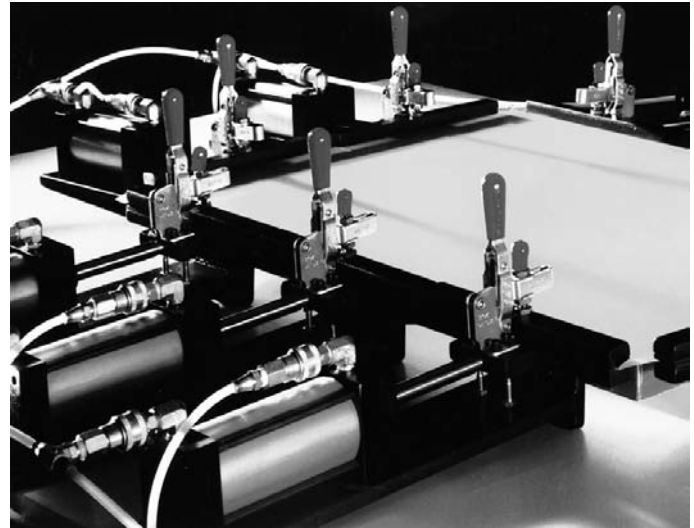
Model 207-U0 hold-down clamps used in fixturing material in a silk screening application.
