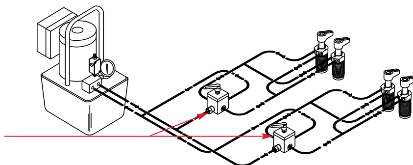
"P" Port Check Valve (500172DE, 500174DE)
