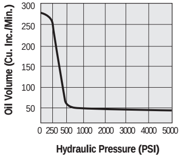
Performance — Pump No. 100186DE
