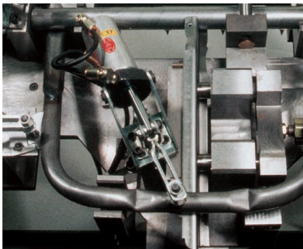
Pneumatic Clamping Technology
