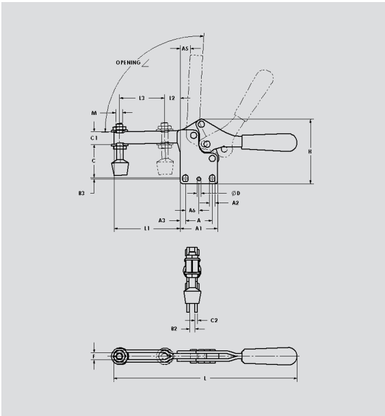
U-shaped clamping bar Straight base
