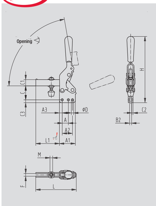
U-bar Straight base
