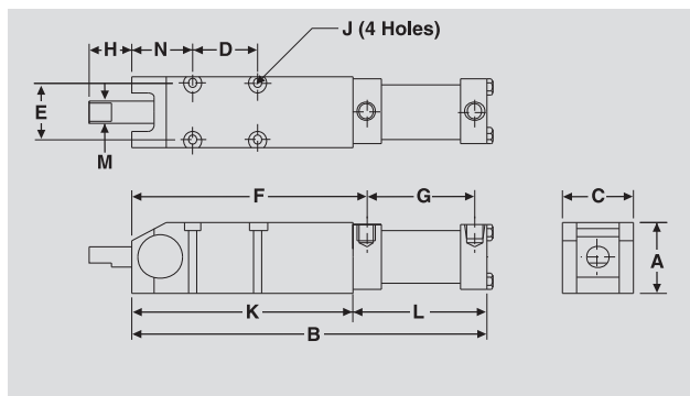
Model 801010 (Arm Extension Option)
