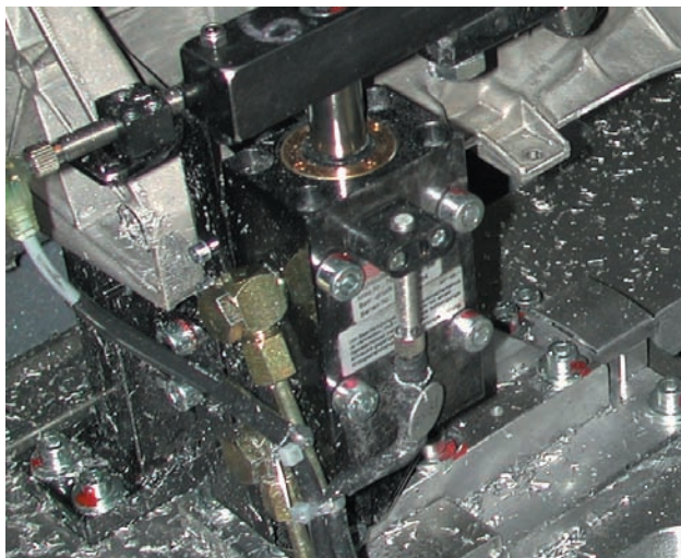
Hydraulic Clamping Technology
