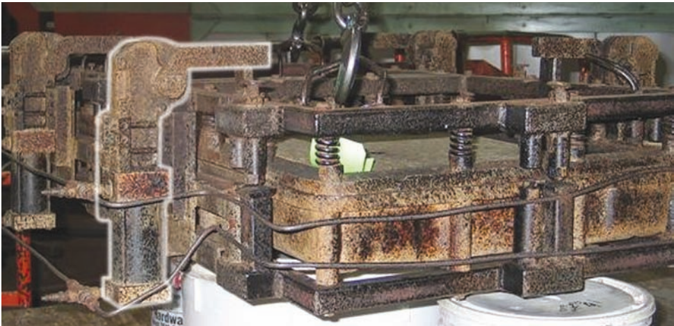
991 MRM clamps (4) used to clamp two mold halves together.
