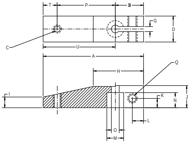
Swing/Pull Clamp Arm
